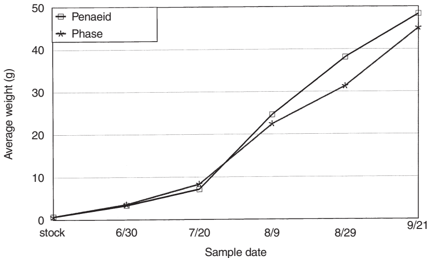
FIGURE 1. Mean sample weights of prawn sampled every three weeks from earthen ponds where prawns were fed either unpelleted distillers' grains with solubles (DDGS) for the first four weeks (22% protein), a 28%-protein prawn diet for weeks 5-12, and a 40%-protein penaeid diet for weeks 13-16 (phase treatment) or a 40%-protein penaeid diet throughout the entire 16-week season (penaeid treatment). Values are means \pm SE of three replicate ponds ( n = 3 ).
